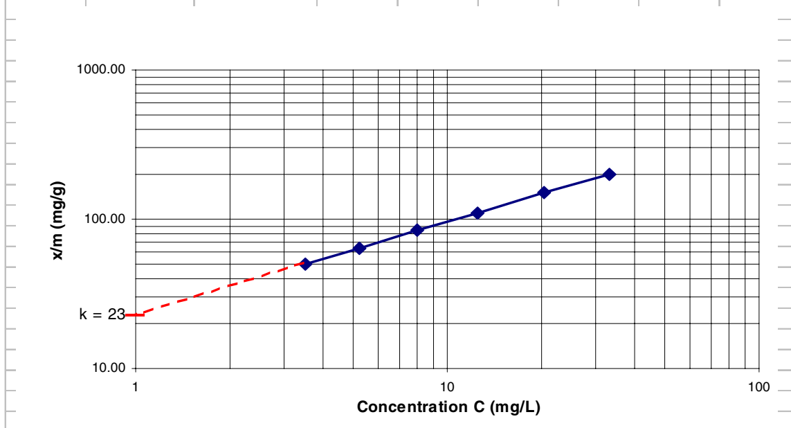
Figure C-2. TOC isotherm and lab data.
