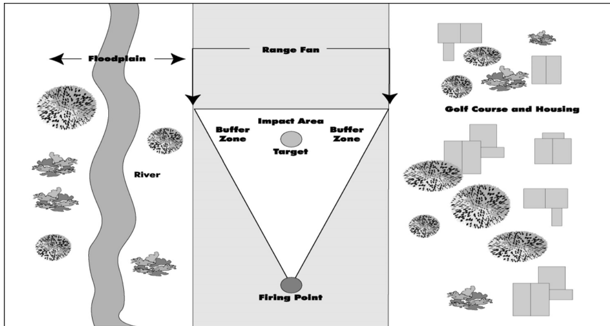
Figure 7-3. Conceptual Site Model: Plan View of a Range Investigation Area
